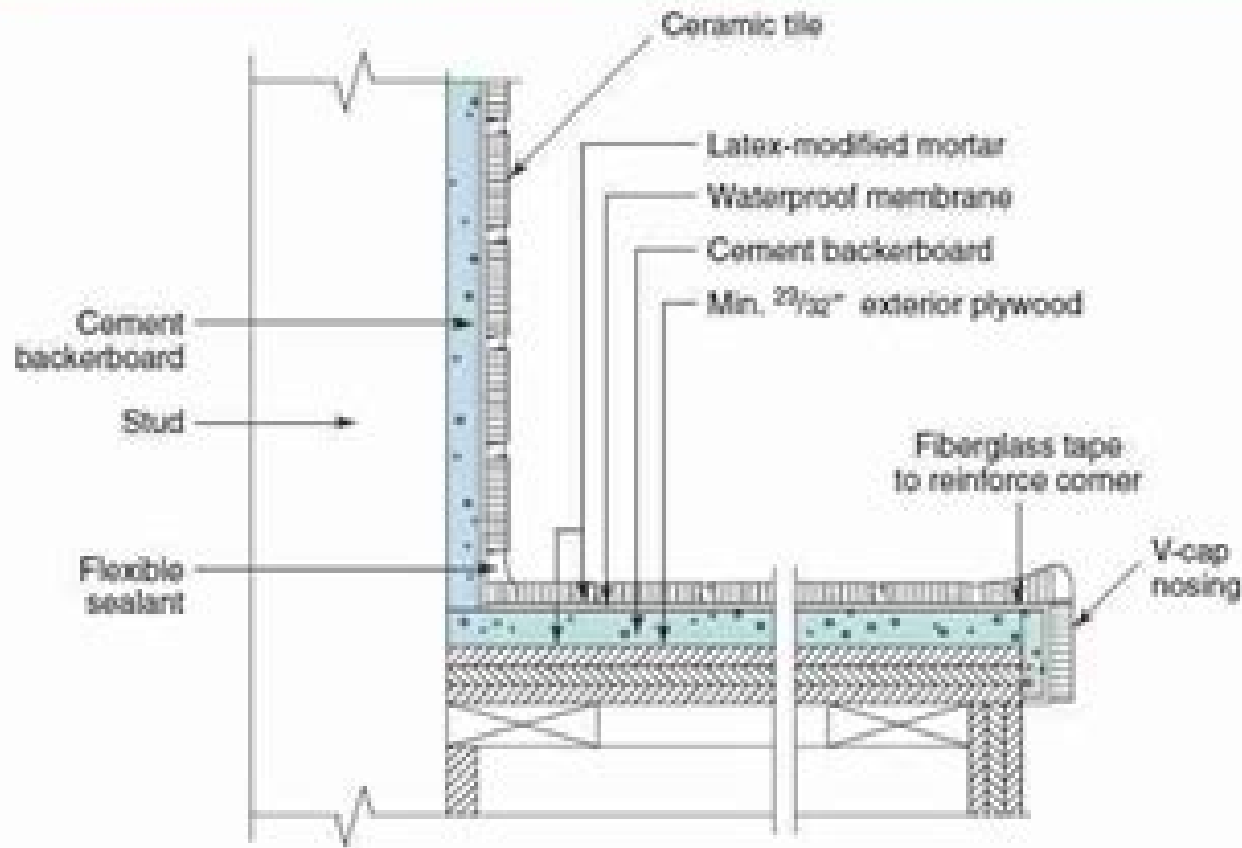
FIGURE 6-35 Wet Counter with Cement Backerboard.
